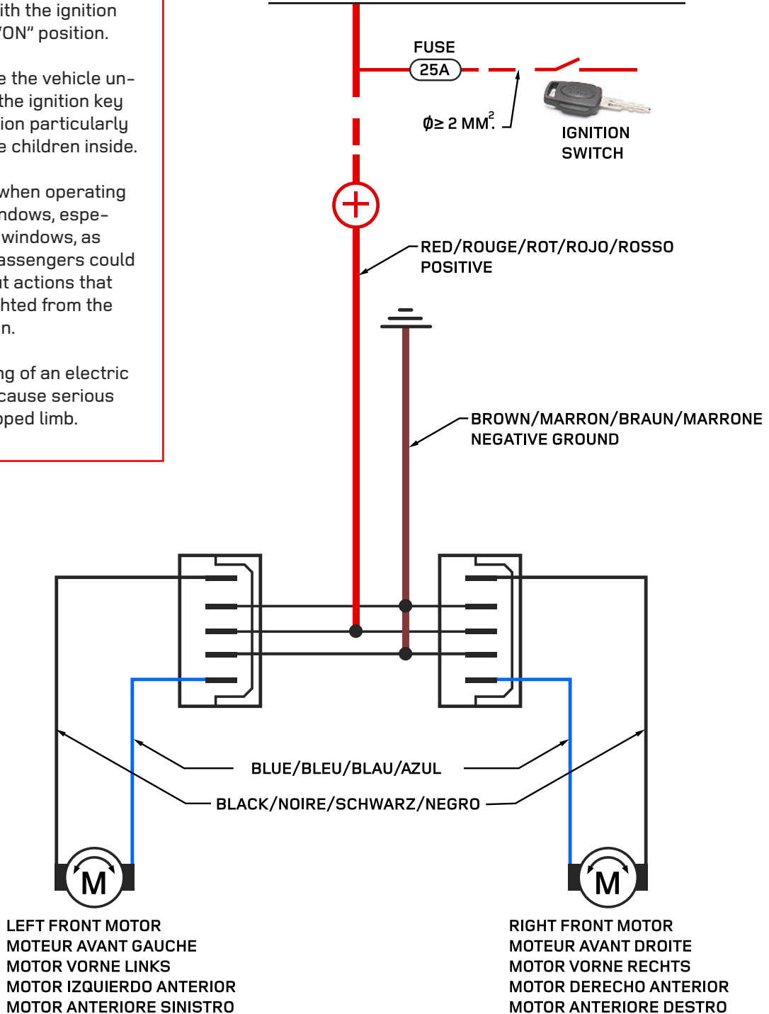
Wiring Diagram
