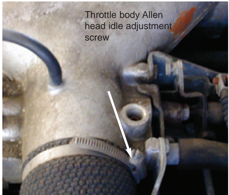
Figure 3. Location of throttle body allen screw adjustment screw, shown with tamper proof plug # RNM109 removed.
